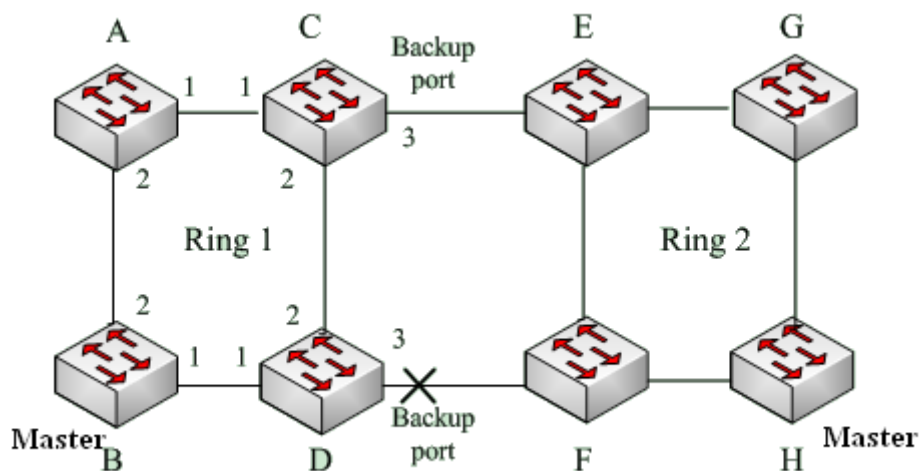
Figure 210 DT-Ring+ Topology
