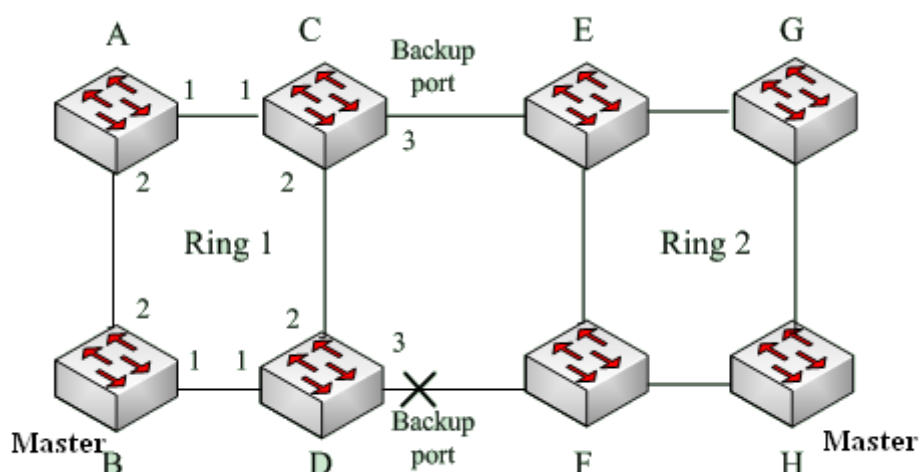
Figure 145 DT-Ring+ Topology
