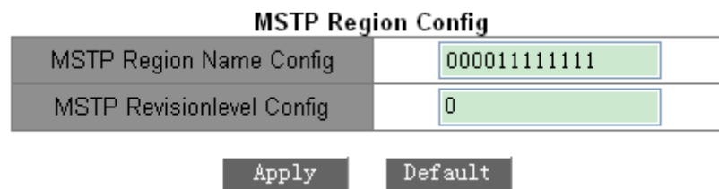
Figure 187 Configuring MST Region Parameters
