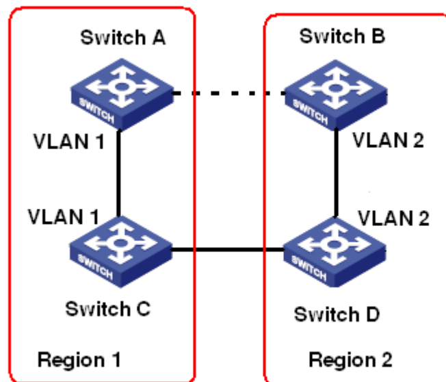
Figure 179 MSTP Topology
