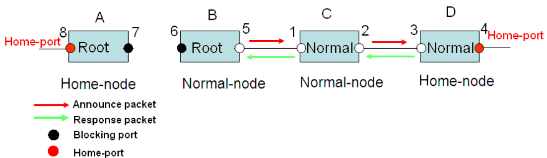
Figure163 DHP Fault Recovery
