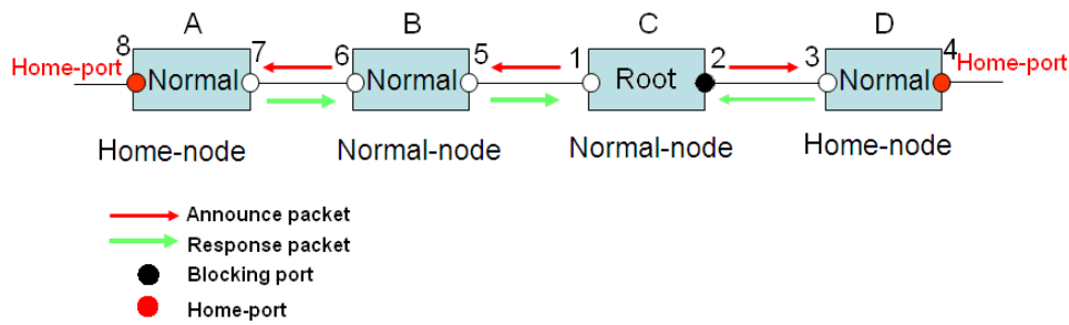
Figure162 DHP Configuration
