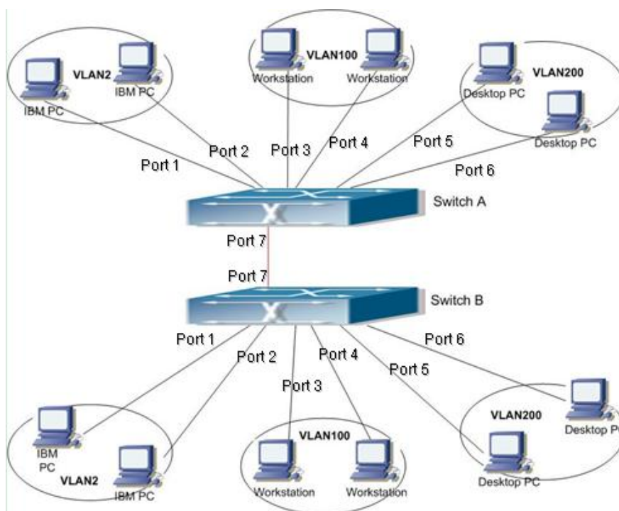
Figure 48 VLAN Application
