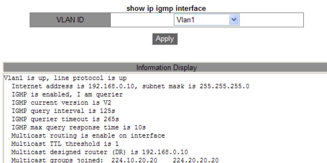
Figure 307 the Information of IP IGMP Interface
