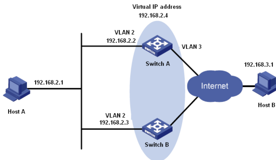
Figure 345 VRRP Typical Configuration Example
