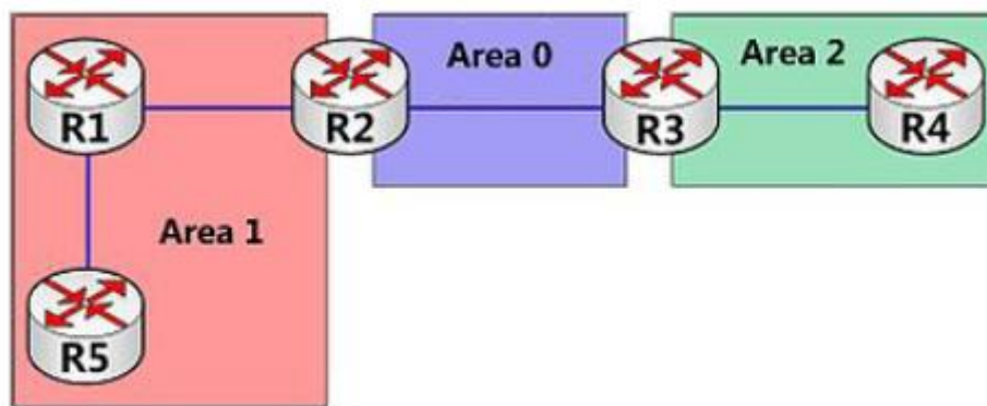
Figure 220 Area Partition
