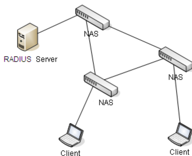
Figure 367 RADIUS Structure
