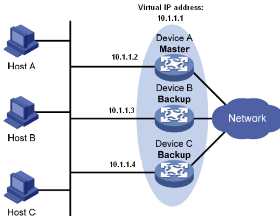
Figure 336 VRRP
