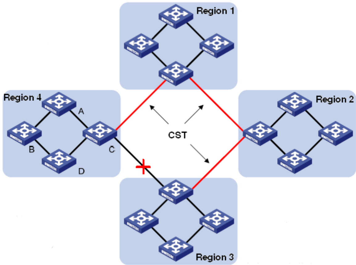
Figure 180 MSTP Concepts
