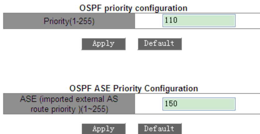
Figure 233 Setting Priorities for Routing Protocol
