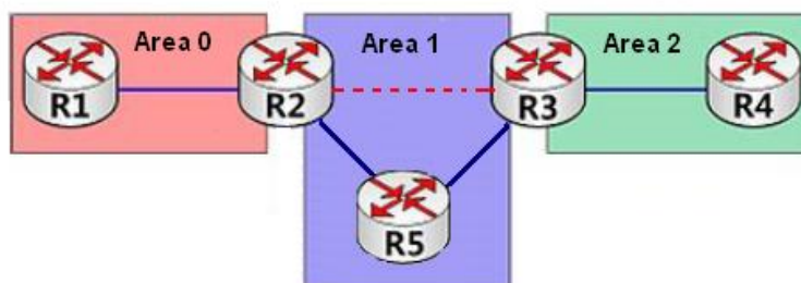
Figure 222 Virtual Link
