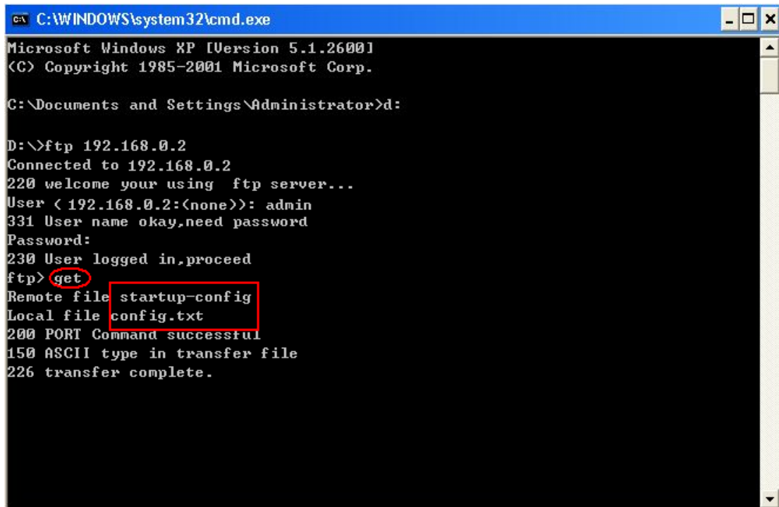
Figure 96 Downloading File from Switch to Client
